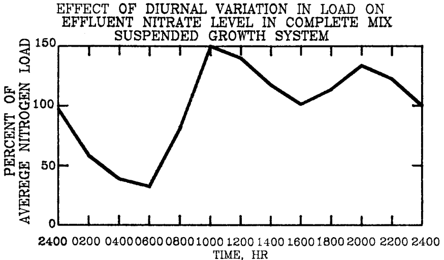
A. ASSUMED VARIATION IN INFLUENT NITROGEN LOAD
