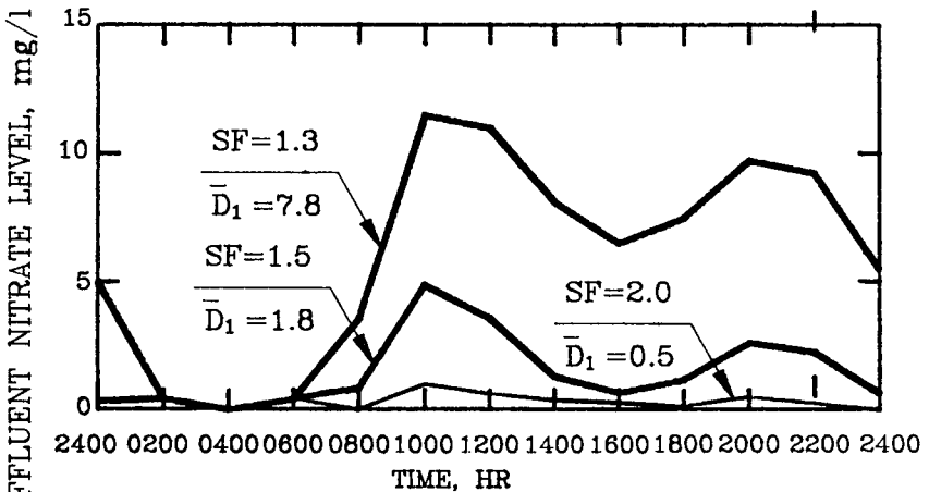
B. CALCULATED EFFLUENT NITRATE LEVEL
